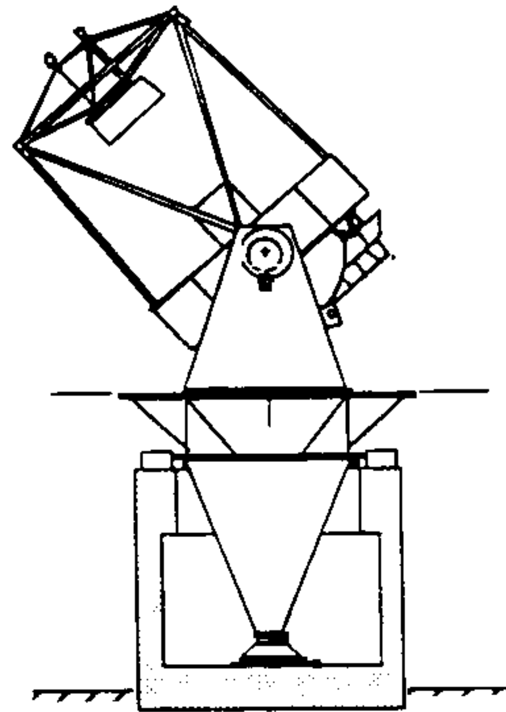
3.5 METER TELESCOPE
