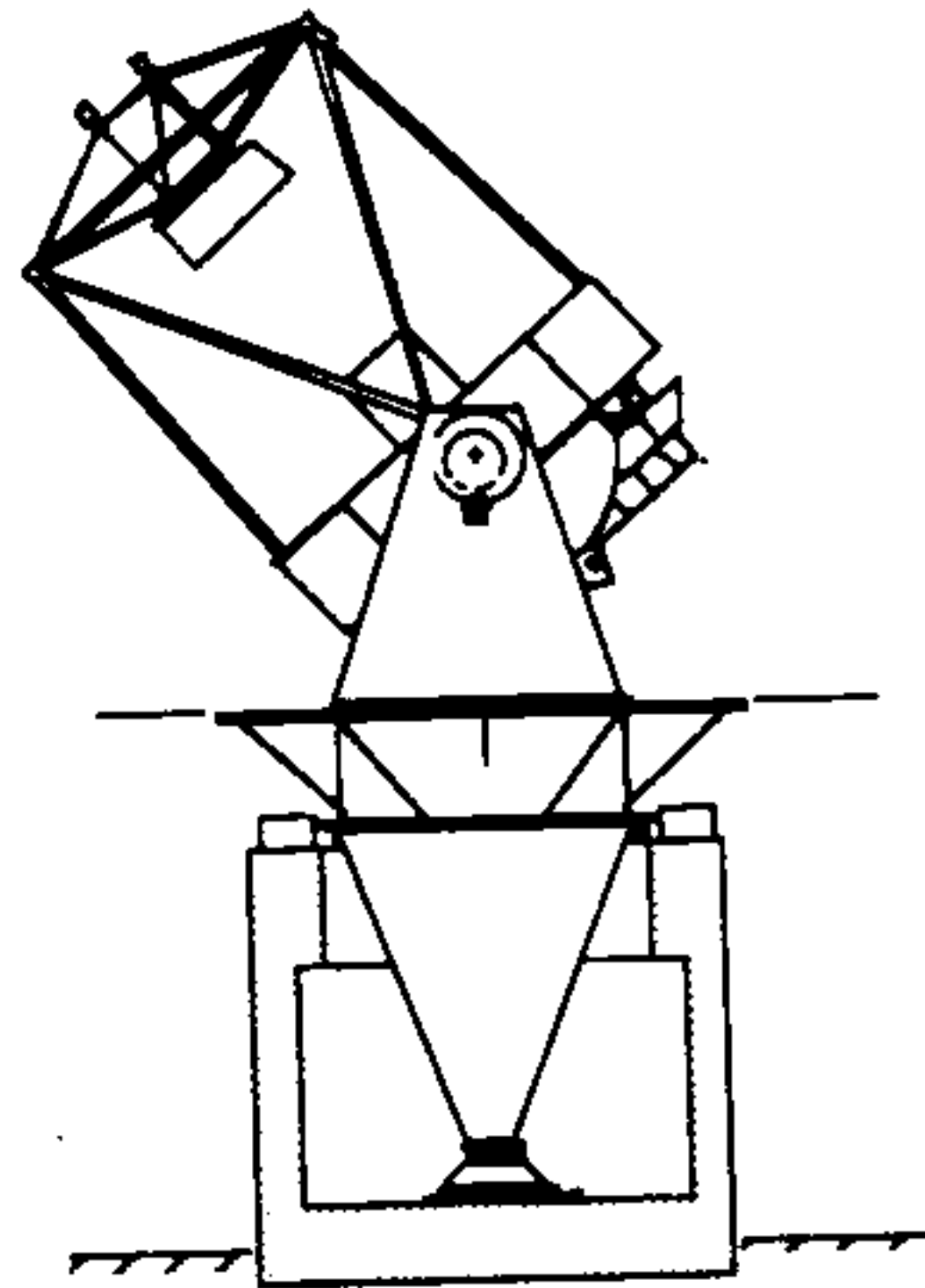
3.5 METER TELESCOPE
