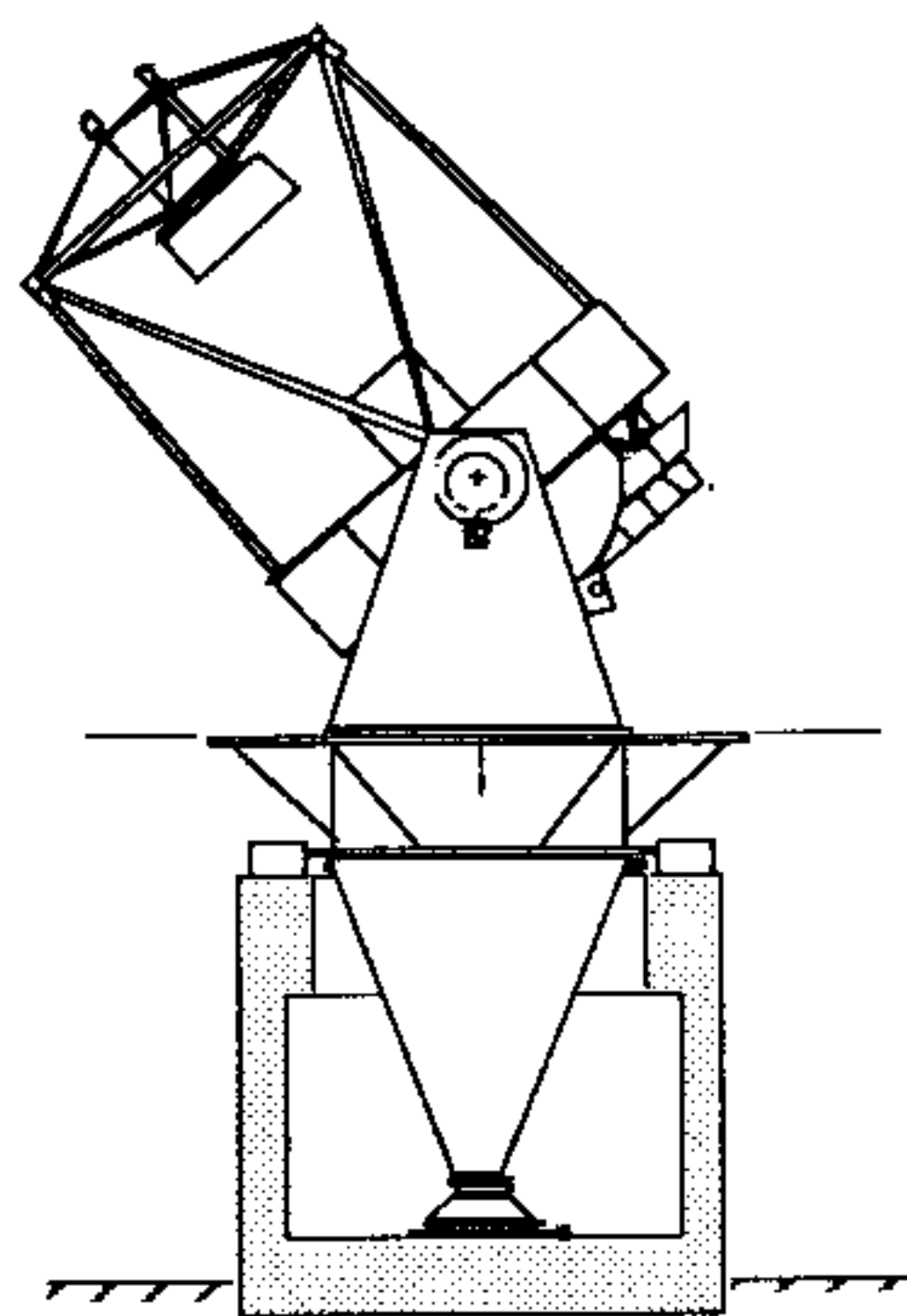
3.5 METER TELESCOPE
